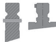
Safety-Pin / Safety-Key Aplicable para pesos de herramienta > 12,5kg/28lbs - < 25kg/56 lbs. (NS I + II) / > 12,5kg/28 lbs - < 150kg/331 lbs (AS II)
