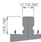
AS II Adaptación American Style II
